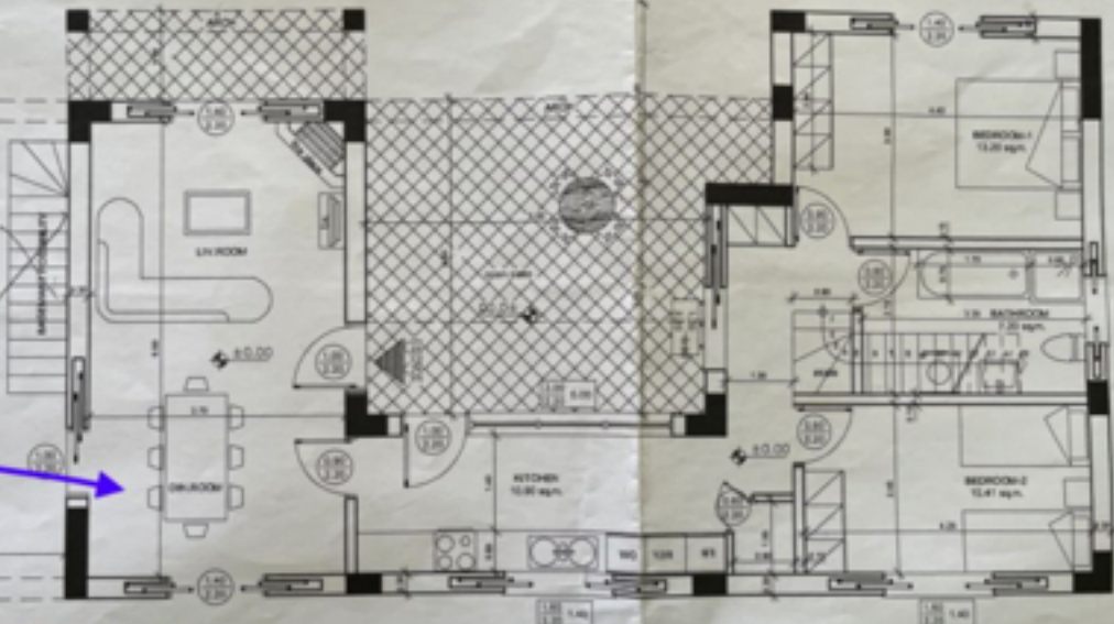
Villa B Ground Floor Plan
